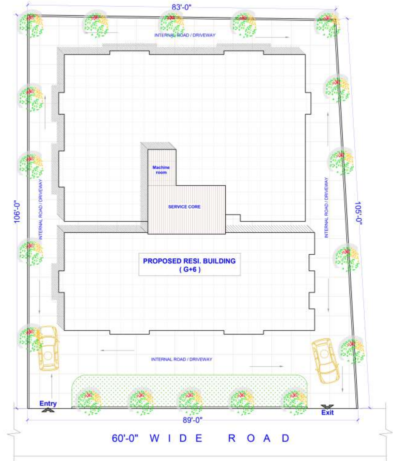
SITE PLAN
